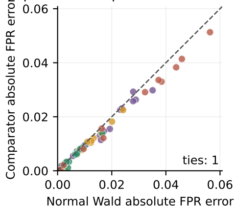
Simple Welch: improved in 53/60 scenarios
